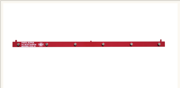
PA-30/39 aileron rigging tool
